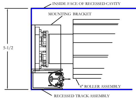
RELATIONSHIP OF U-CHANNEL TO MOTOR BRACKET IN A MINIMUM RECESSED CAVITY C/W 4" ROLLER
